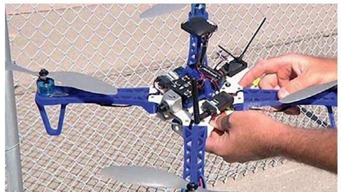
Figure 21: US Navy's 3D-printed drone; Source: 3ders
